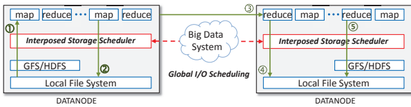
Figure 1: Architecture of IBIS
