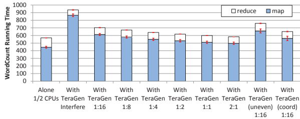
Figure 2: Runtime of WordCount without/with IBIS with varying I/O sharing ratios (WC:TG)
